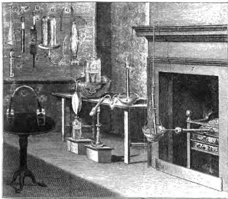
PRIESTLEY'S LABORATORY
